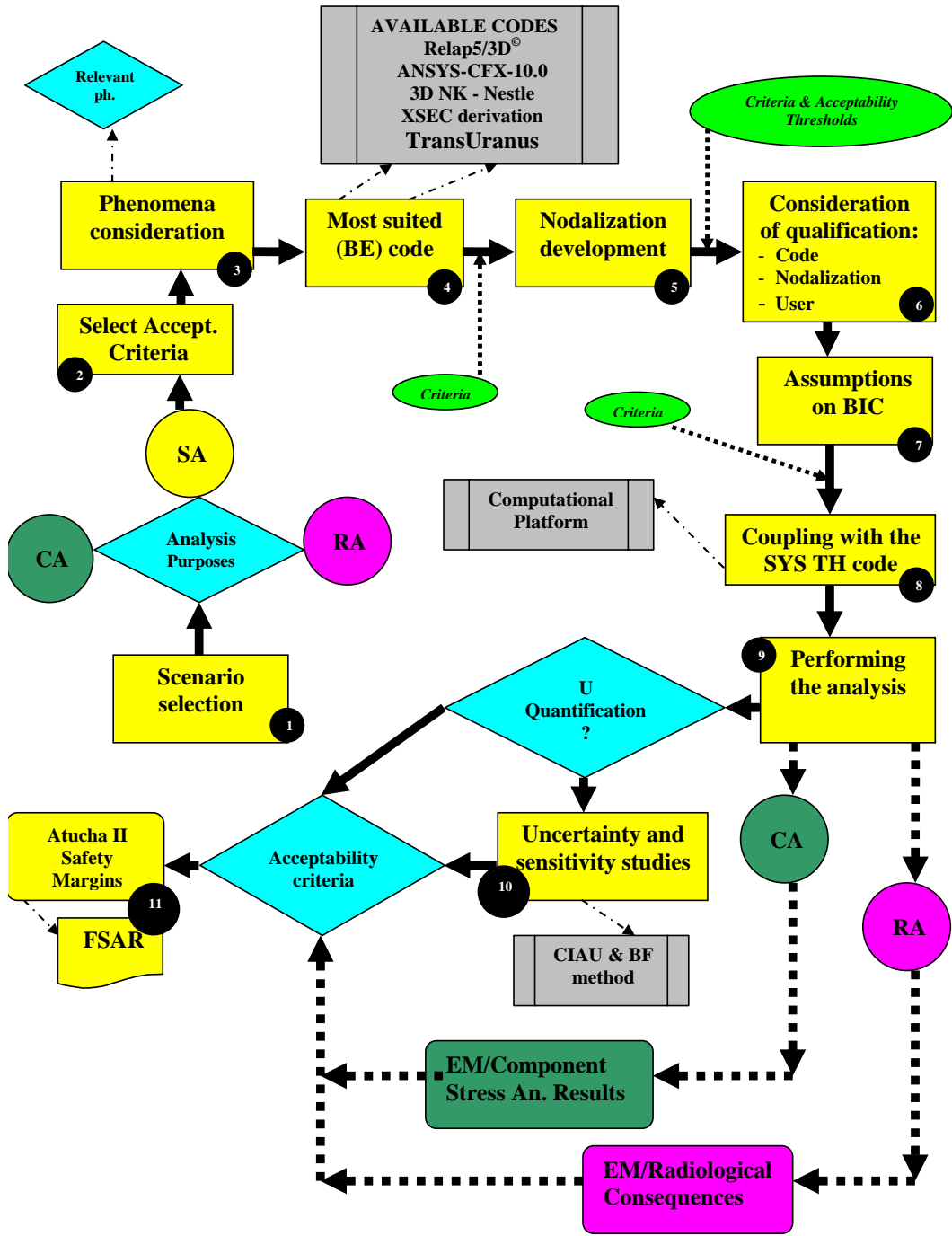
Fig. 1. The BEPU flow-diagram.
