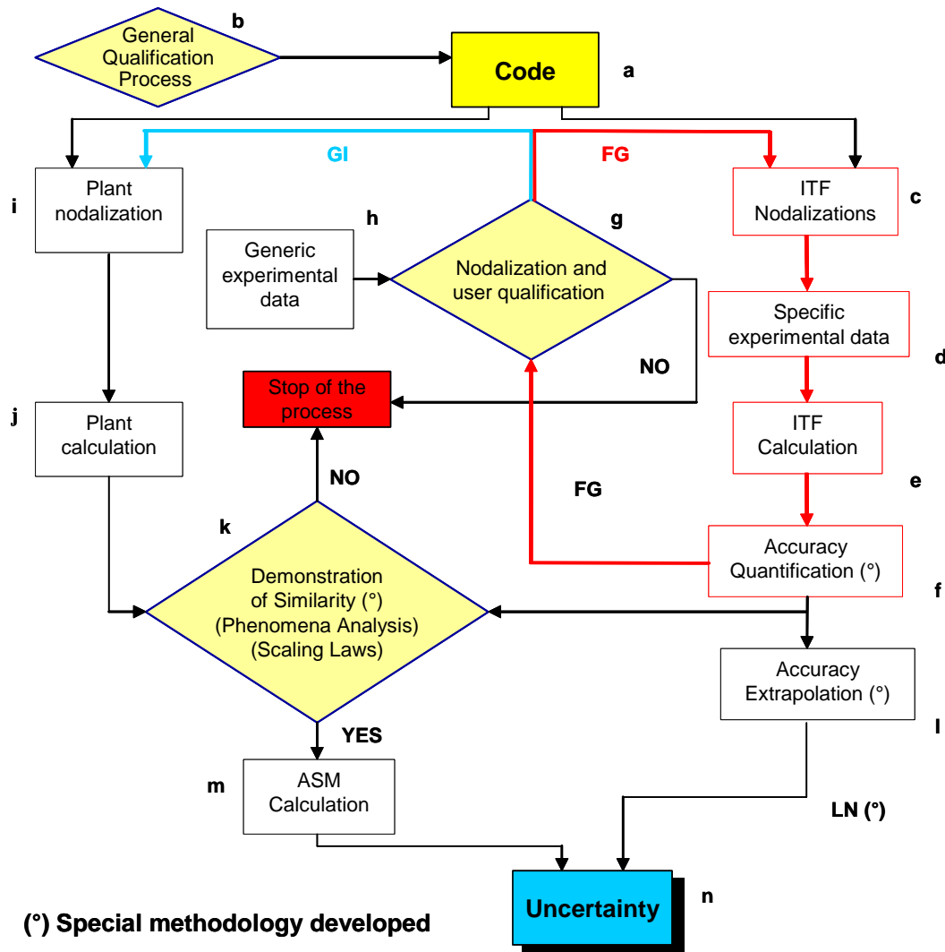
Fig. 3. The flow-diagram of UMAE.
