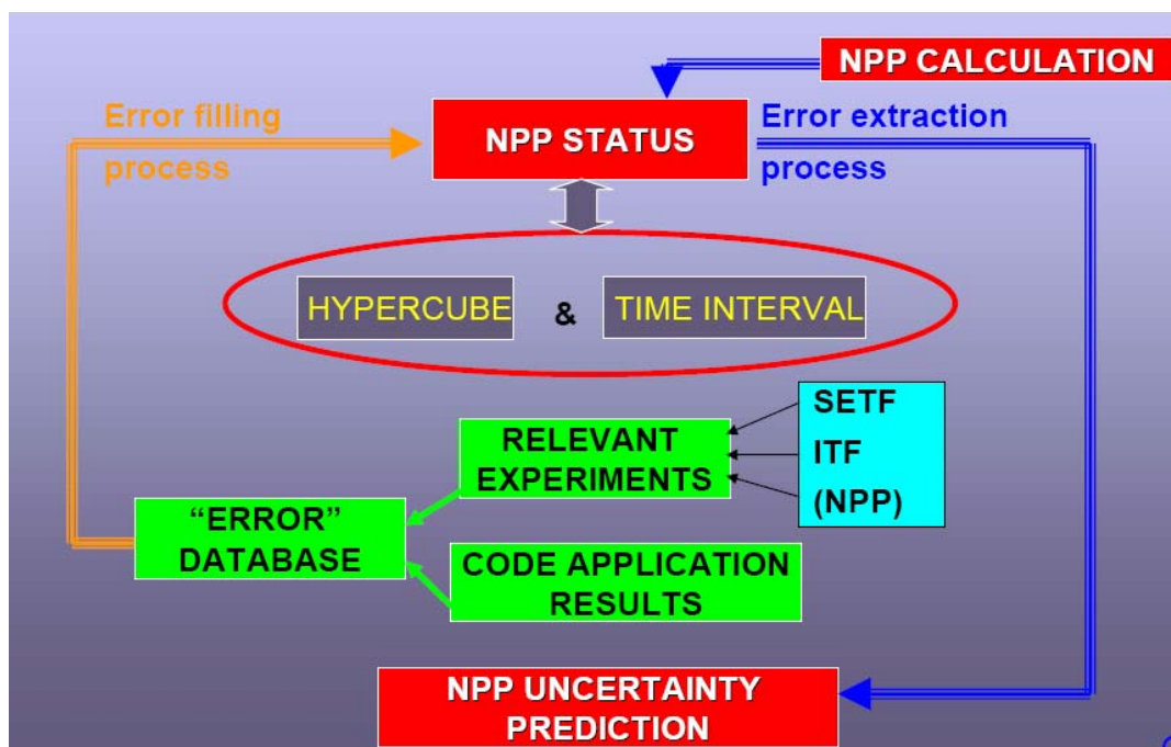
Fig. 4. Outline of the basic idea of the CIAU method.
